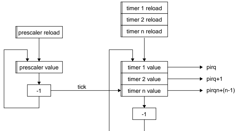
Figure 128. General Purpose Timer Unit block diagram
