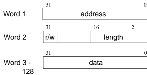
Figure 293. Layout of USB DCL write commands.
