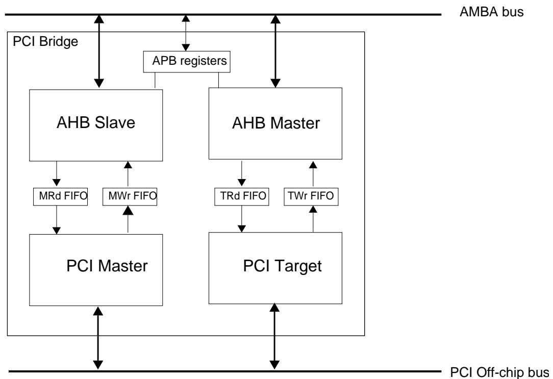
Figure 240. GRPCI master/target
