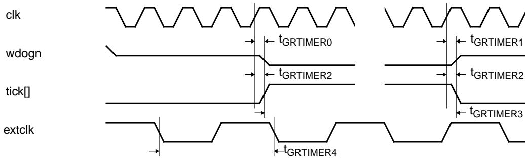
Figure 138. Timing waveforms
