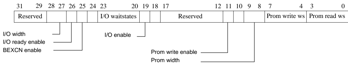
Figure 285. Memory configuration register
