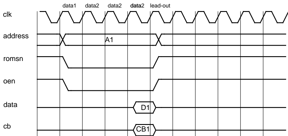
Figure 225. Prom read access with two waitstates.
