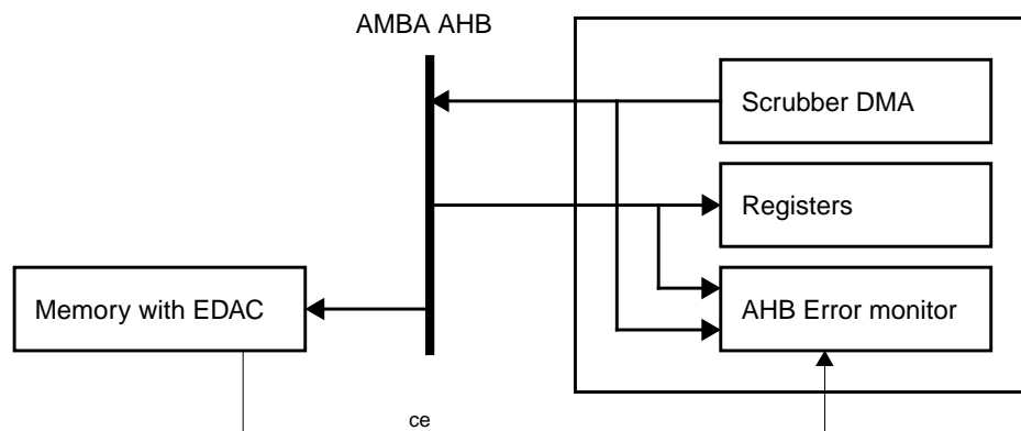
Figure 238. Memory scrubber block diagram
