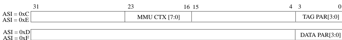
Figure 202. Data cache tag diagnostic access when CCR.PS = ‘1’
