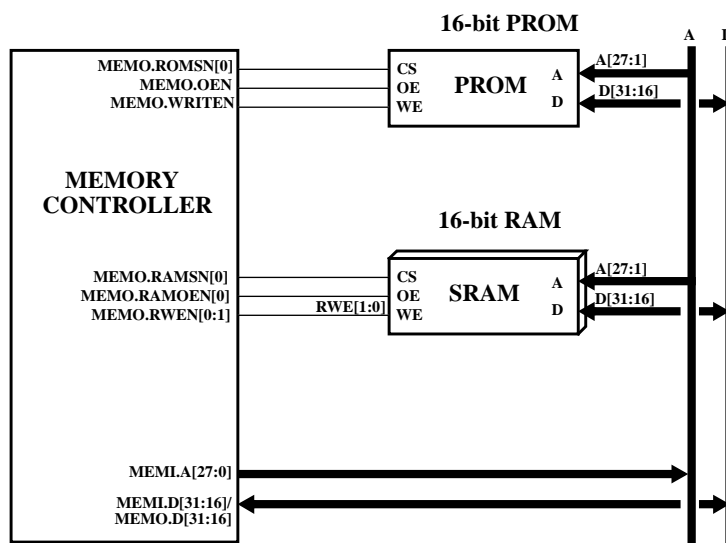
Figure 233. 16-bit memory interface example
