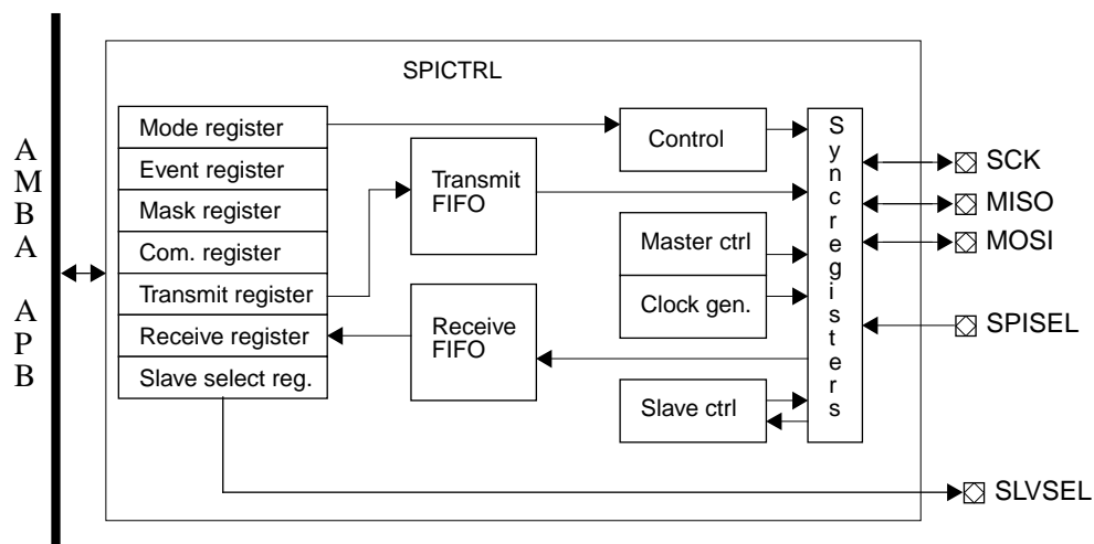
Figure 272. Block diagram
