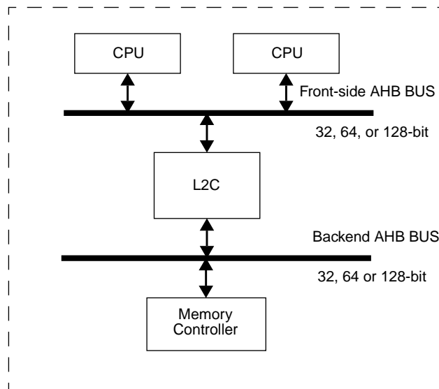
Figure 187. Block diagram
