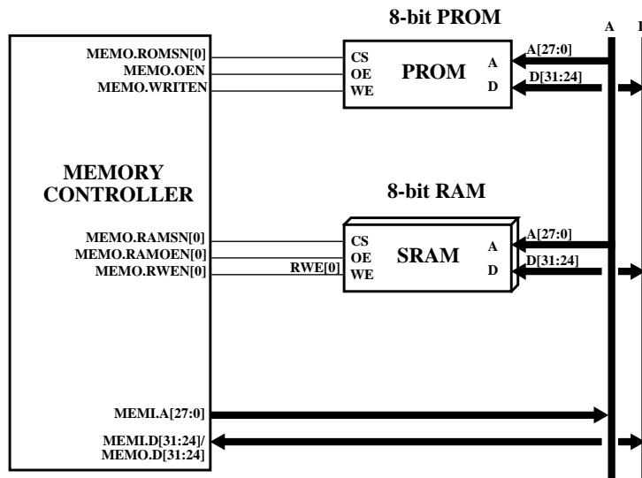
Figure 232. 8-bit memory interface example
