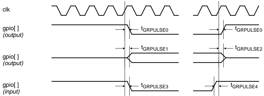
Figure 157. Timing waveforms
