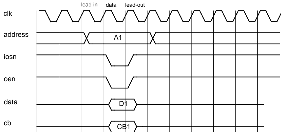
Figure 229. I/O write cycle (0-waitstates)
