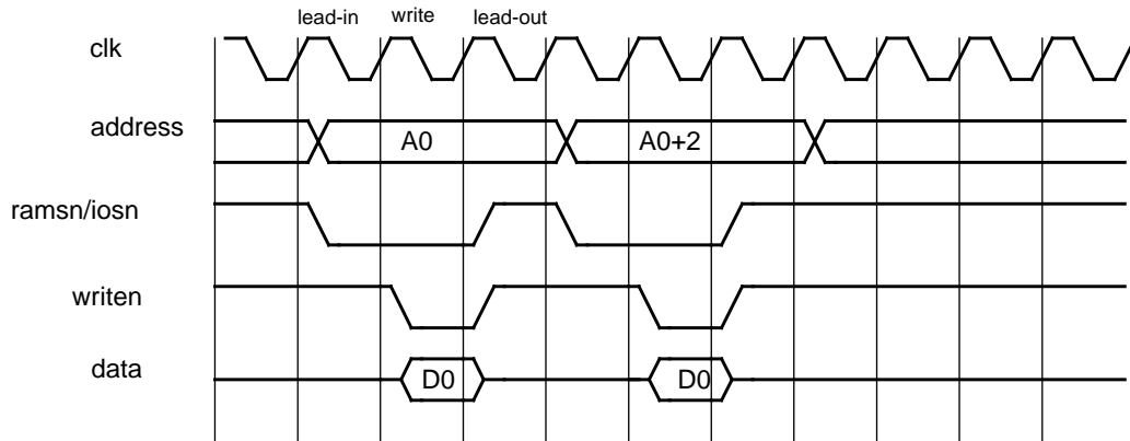
Figure 284. 32-bit PROM/I/O write cycle in 16-bit mode
