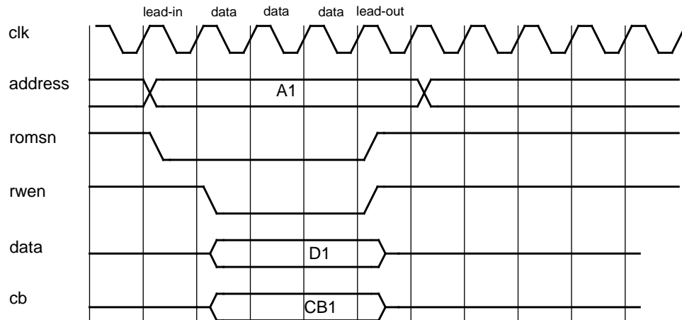
Figure 227. Prom write cycle (2-waitstates)
