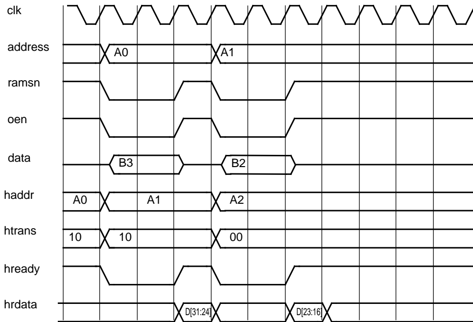
Figure 123. 8-bit SRAM non-sequential read access with 0 wait-states and EDAC enabled.
