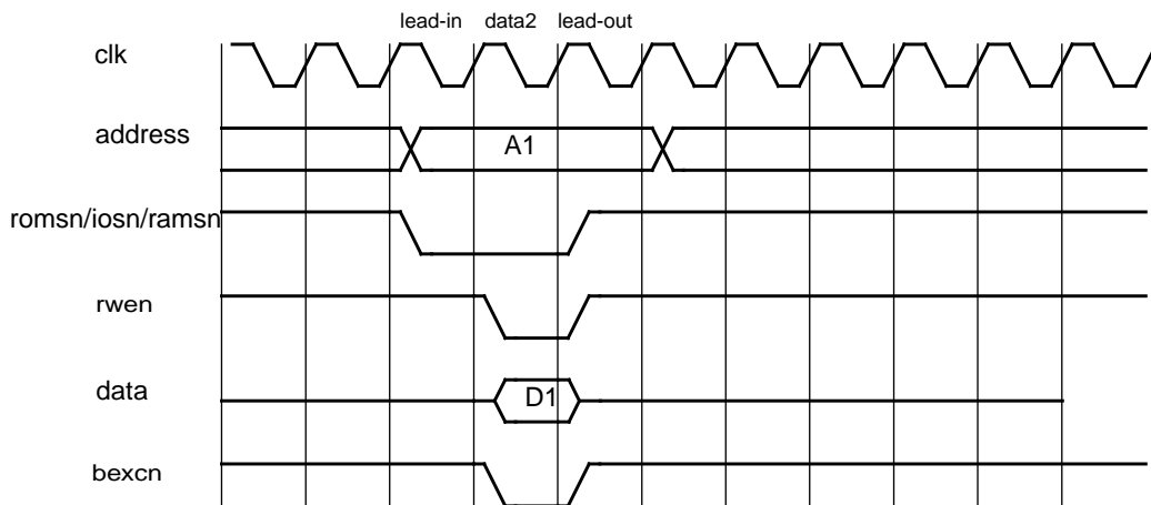
Figure 237. Write cycle with BEXCN. Chip-select (iosn) is not asserted in lead-in cycle for io-accesses.
