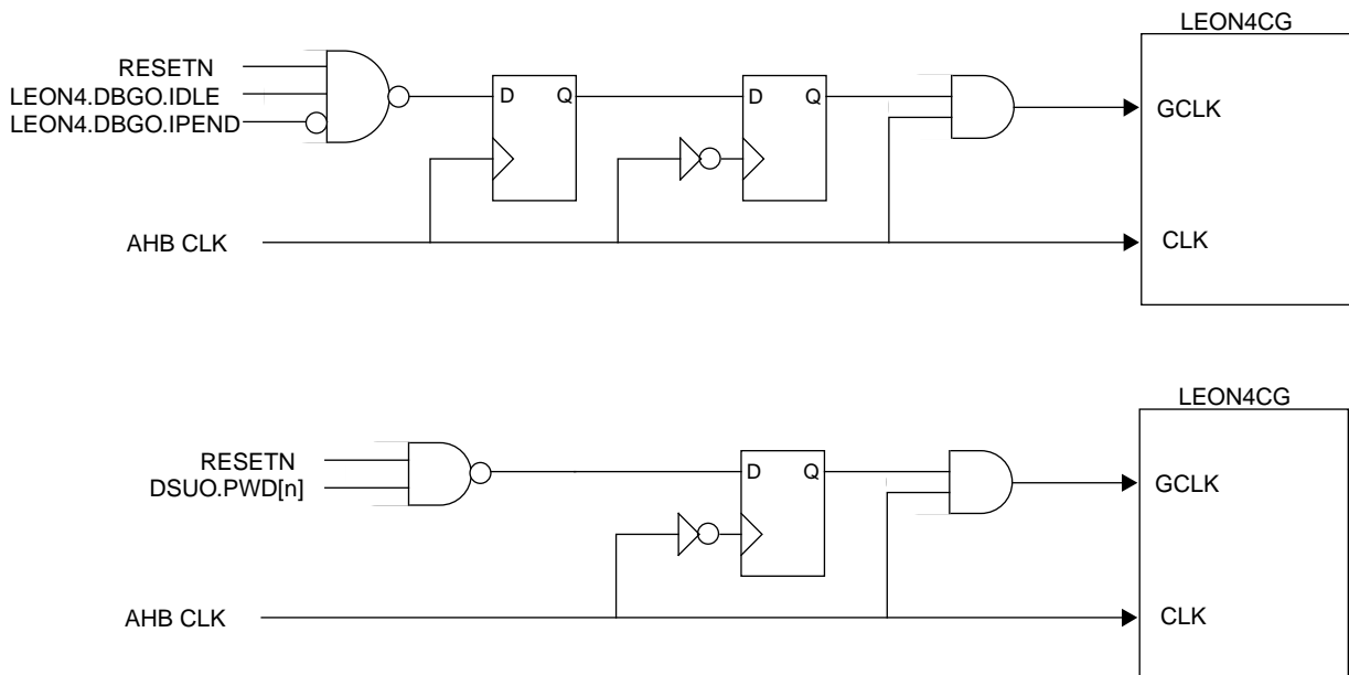
Figure 213. Examples of LEON4 clock gating
