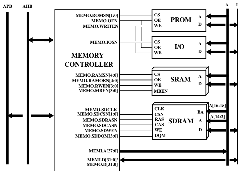
Figure 222. Memory controller connected to AMBA bus and different types of memory devices
