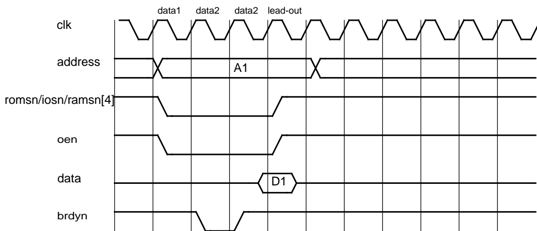
Figure 234. READ cycle with one extra data2 cycle added with BRDYN (synchronous sampling). Lead-out cycle is only applicable for I/O accesses.
