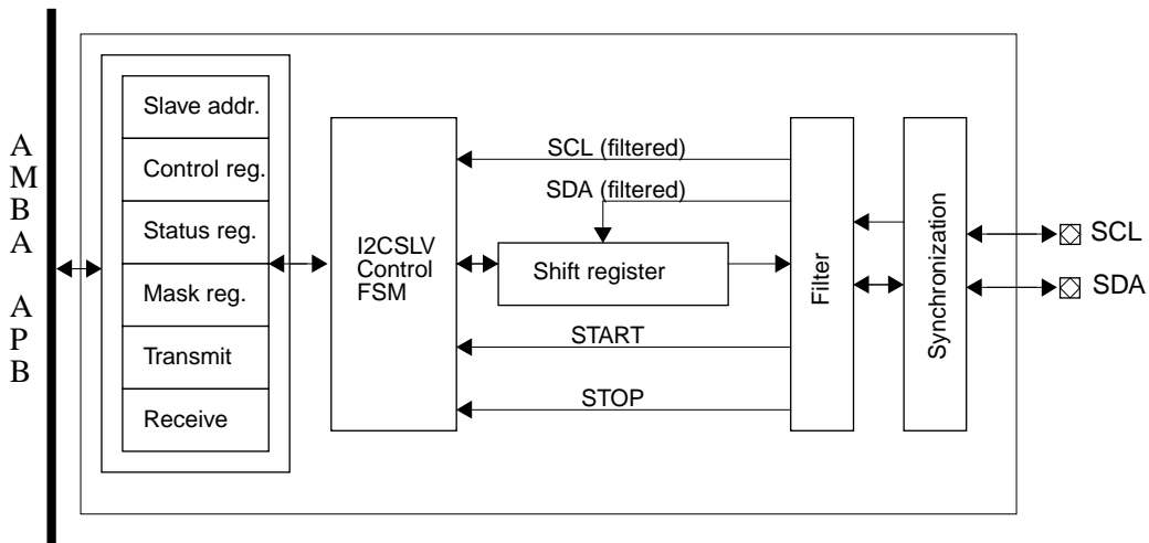
Figure 181. Block diagram
