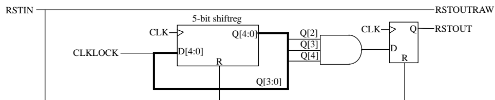
Figure 267. Reset generator with VHDL generic syncrst set to 0 and scan test disabled
