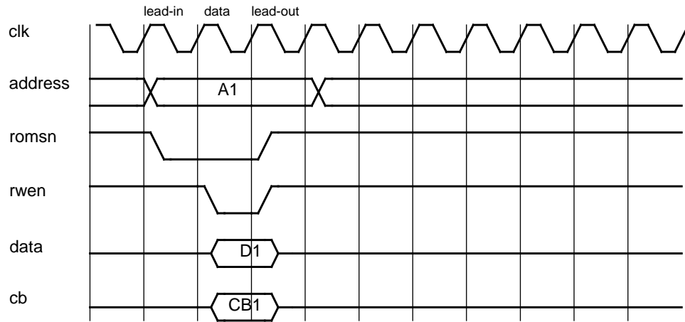
Figure 226. Prom write cycle (0-waitstates)
