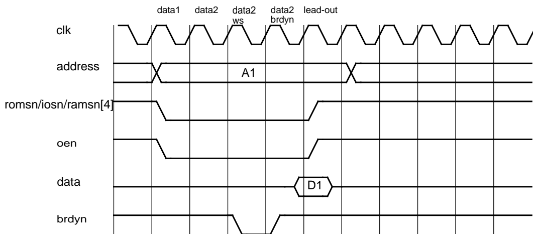
Figure 235. Read cycle with one waitstate (configured) and one BRDYN generated waitstate (synchronous sampling).
