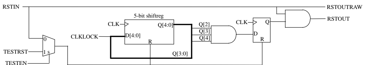
Figure 268. Reset generator with VHDL generic syncrst set to 0 and scan test enabled
