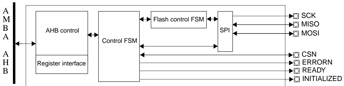
Figure 274. Block diagram
