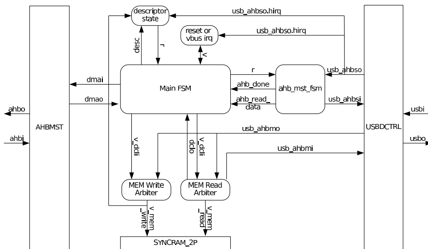
Figure 291. Block diagram of the internal structure of the GRUSBDCCL. Blocks with rounded corners are implemented as VHDL procedures while squares represent VHDL entities.
