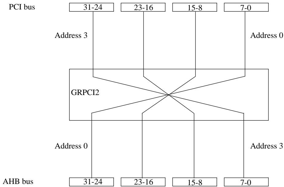
Figure 257. GRPCI2 byte twisting
