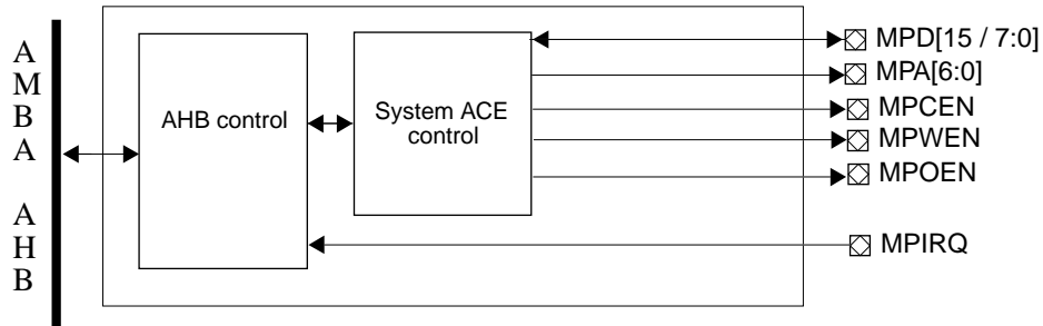
Figure 139. Block diagram
