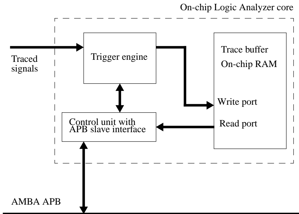
Figure 214. On-chip Logic Analyzer block diagram
