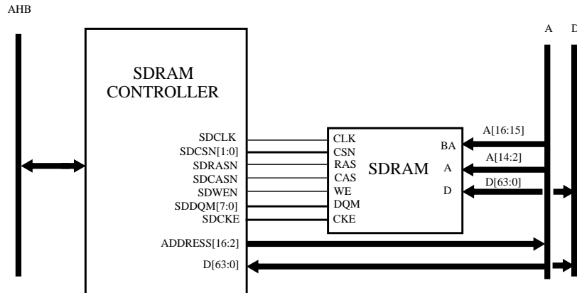
Figure 269. SDRAM Memory controller connected to AMBA bus and SDRAM
