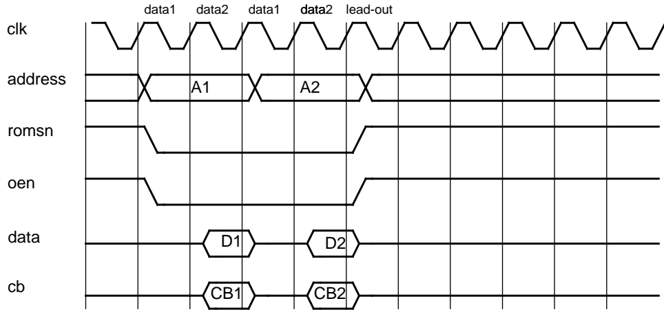
Figure 224. Prom consecutive read cycles.
