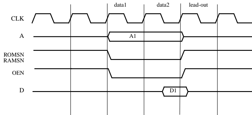
Figure 276. 32-bit PROM/SRAM/IO read cycle
