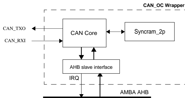
Figure 42. Block diagram
