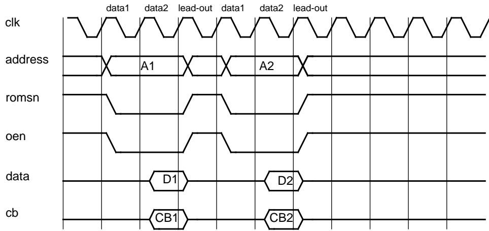
Figure 223. Prom non-consecutive read cycles.
