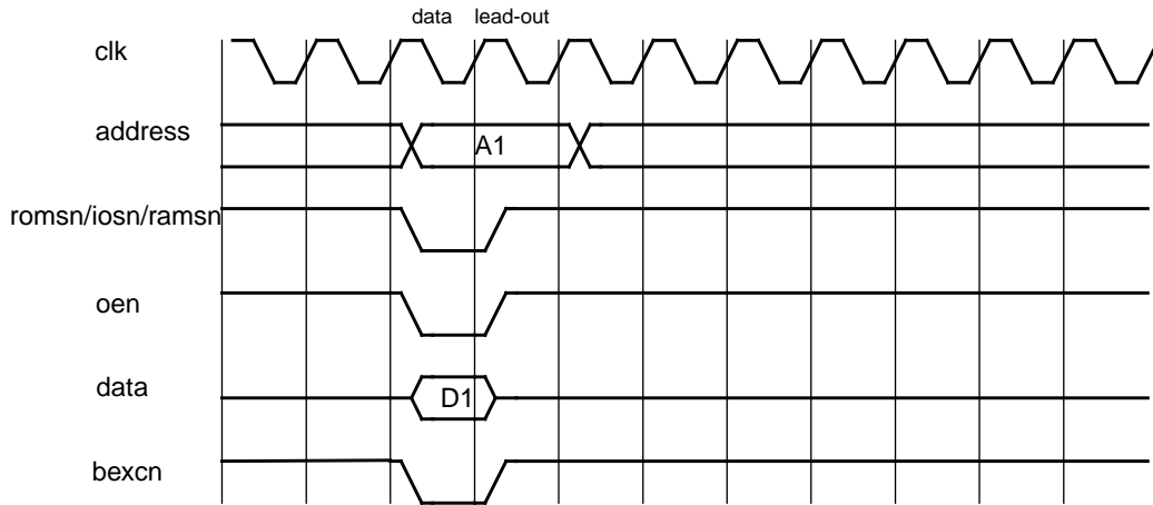
Figure 106. Read cycle with BEXCN.
