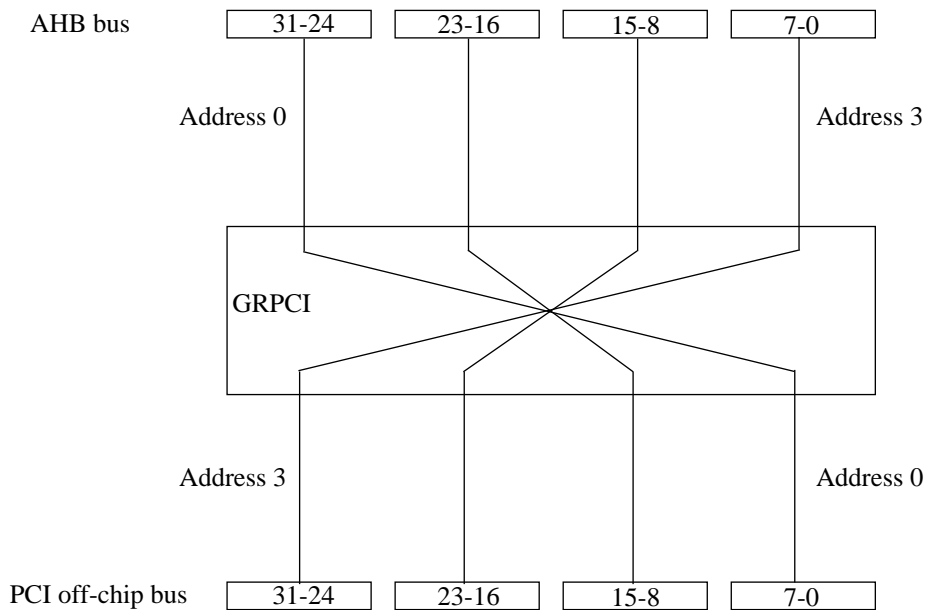
Figure 252. GRPCI byte twisting
