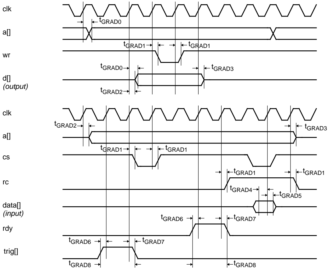
Figure 152. Timing waveforms
