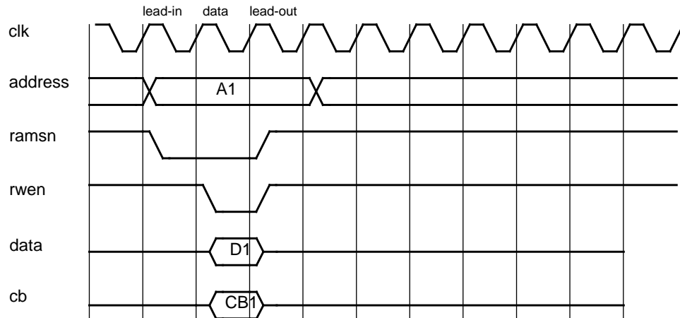
Figure 231. Sram write cycle (0-waitstates)
