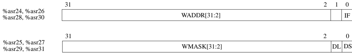
Figure 205. Watch-point registers
