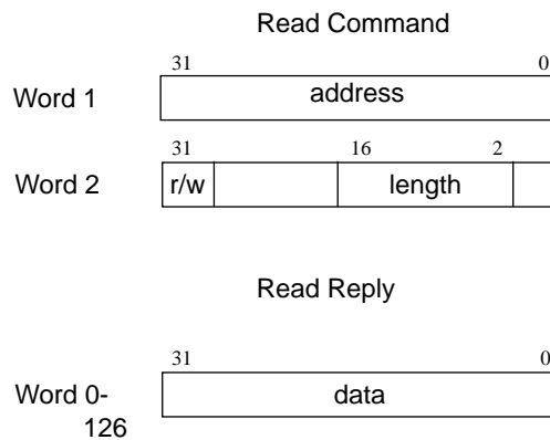
Figure 294. Layout of USB DCL read commands and replies.
