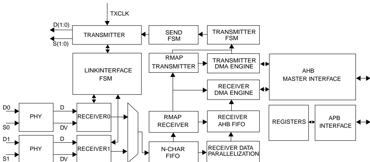
Figure 166. Block diagram
