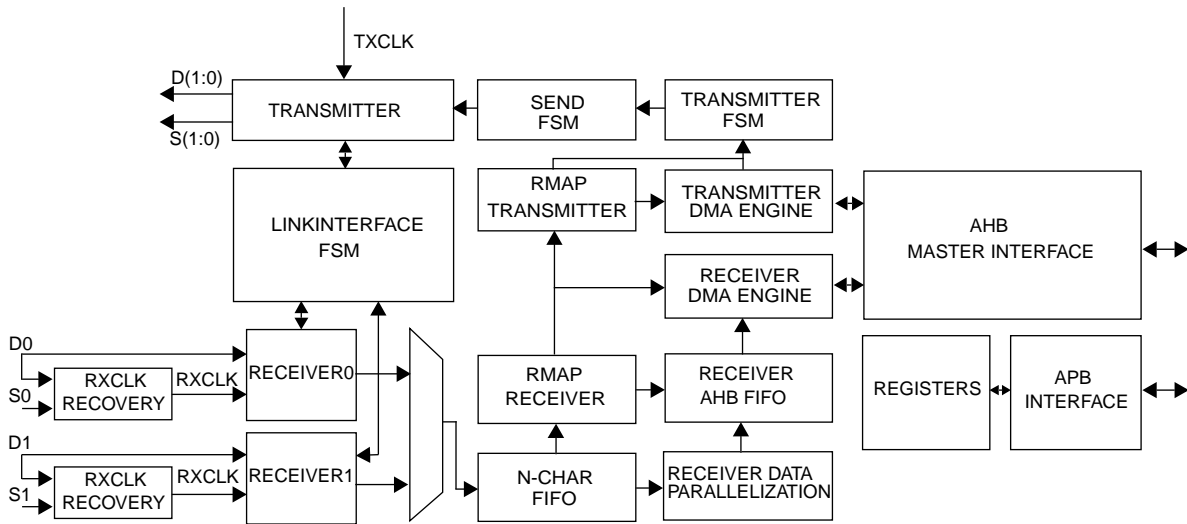
Figure 159. Block diagram
