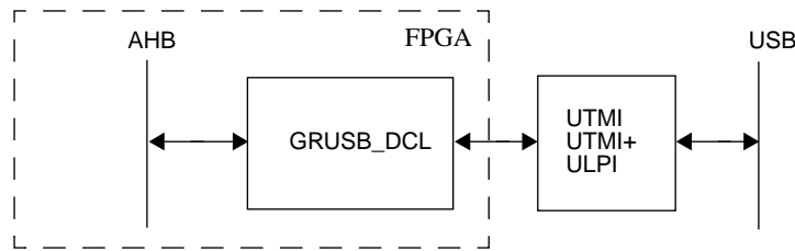
Figure 290. USBDCCL connected to an external UTM.
