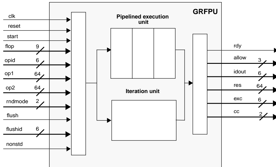
Figure 153. GRFPU Logical View
