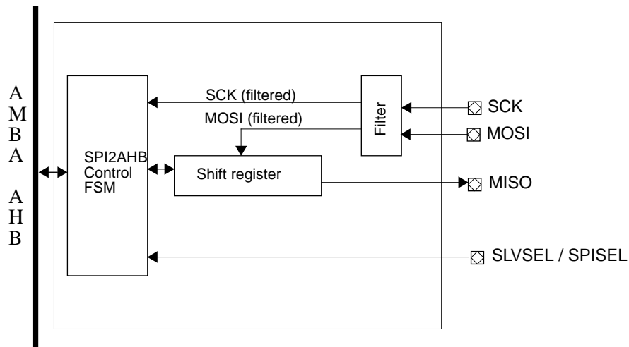
Figure 270. Block diagram, optional APB interface not shown
