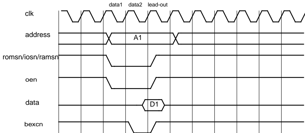
Figure 236. Read cycle with BEXCN.
