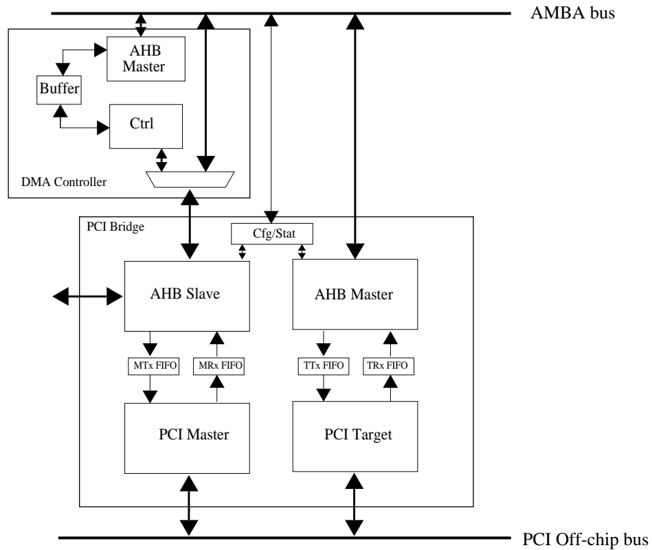
Figure 258. DMA Controller unit
