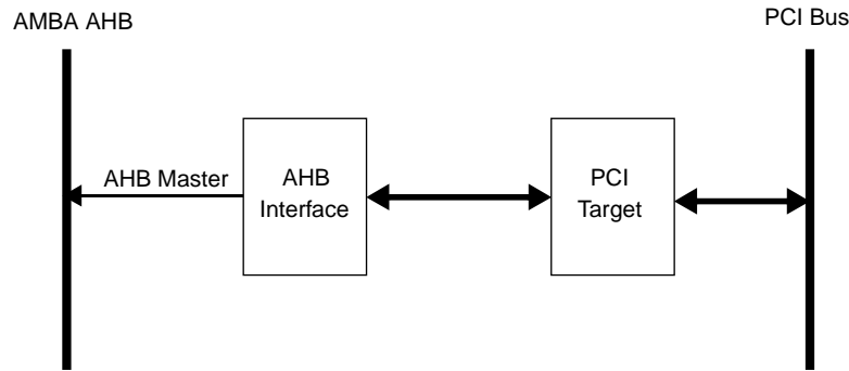
Figure 263. Target-only PCI interface
