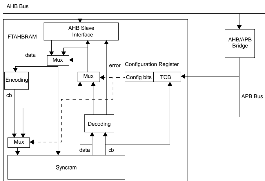
Figure 82. Block diagram
