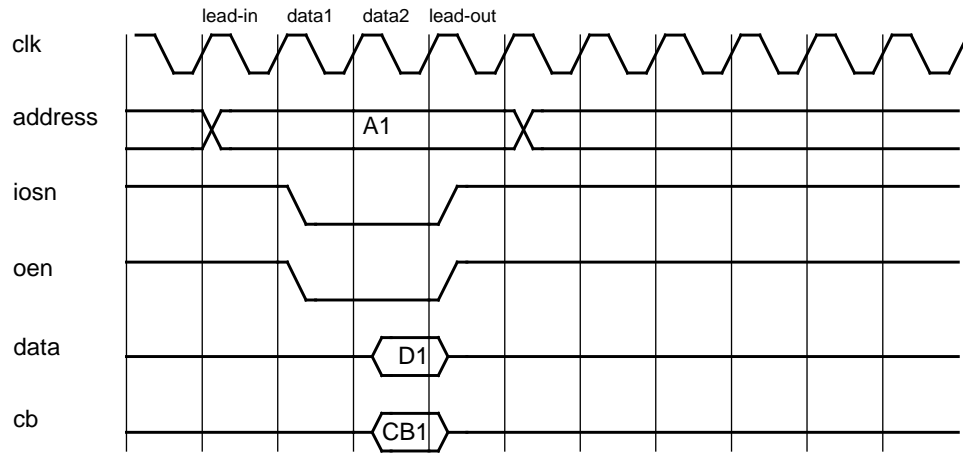
Figure 228. I/O read cycle (0-waitstates)
