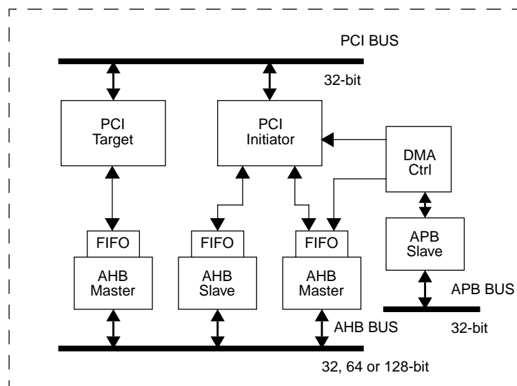
Figure 256. Block diagram
