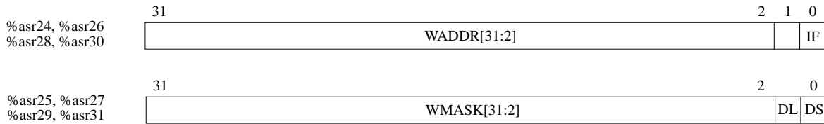
Figure 190. Watch-point registers
