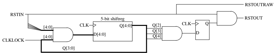
Figure 266. Reset generator with VHDL generic syncrst set to 1
