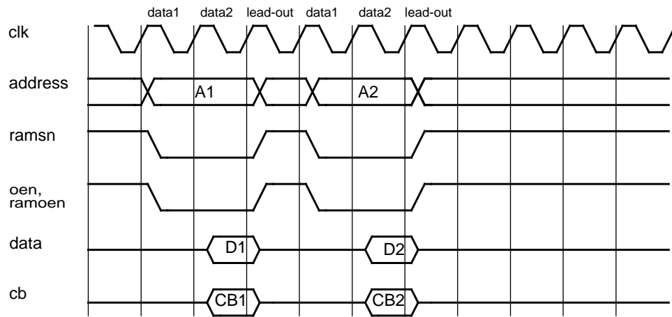
Figure 230. SRAM non-consecutive read cycles.
