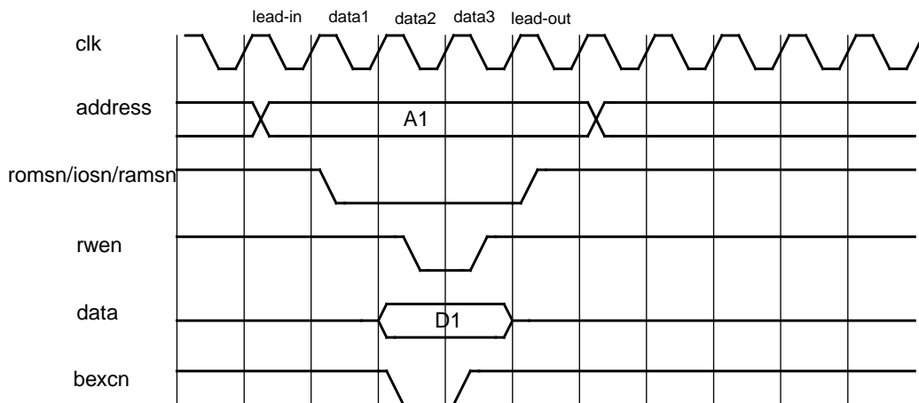
Figure 107. Write cycle with BEXCN.
