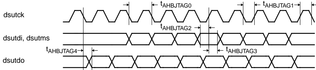
Figure 6. Timing waveforms
